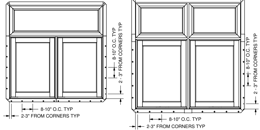
HEAD, SILL & SIDE ANCHORAGE TYPICAL
